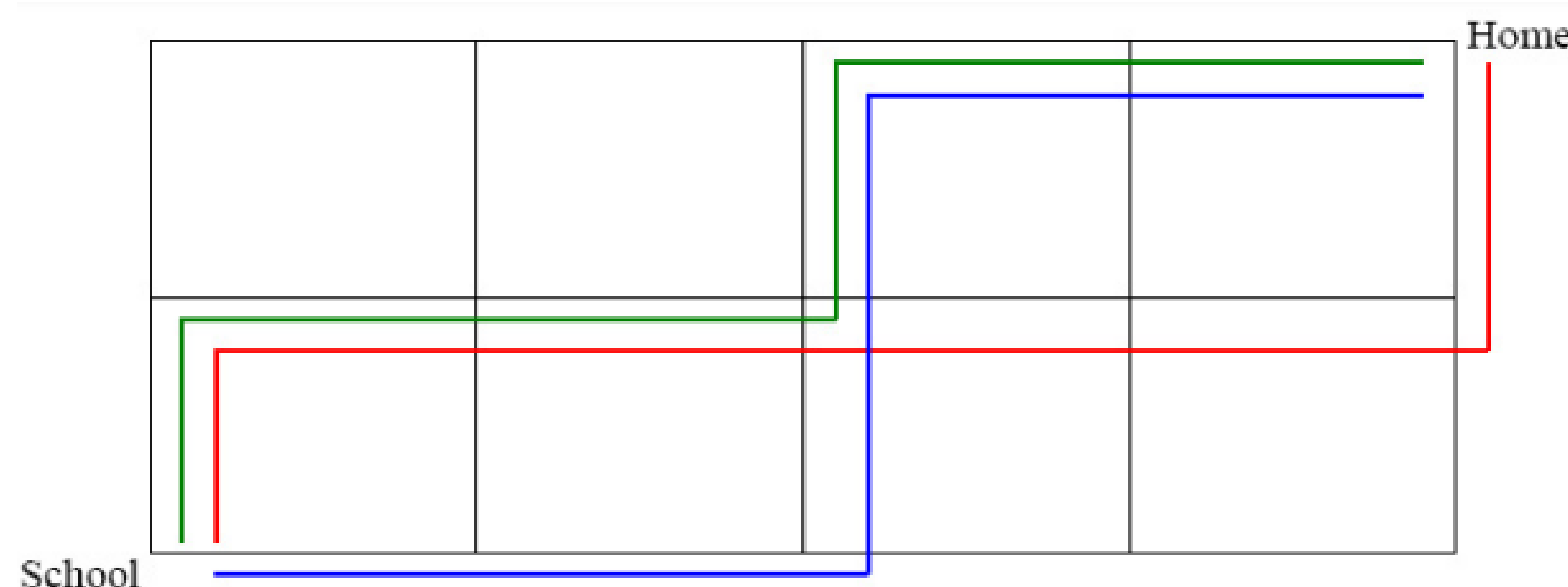
Figure 1. Sample m \times n = 4 \times 2 lattice. Each edge is a street with a different landmark. These three paths are 4-distinct because any two paths share fewer than 4 edges.
