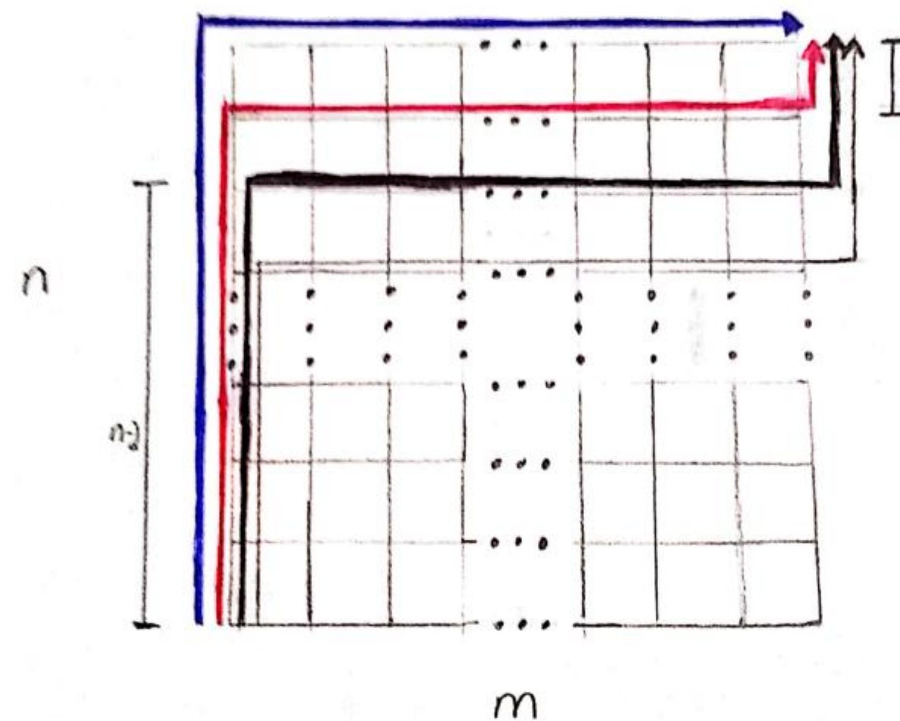
Figure 2. Visual proof of Theorem 1. The n+1 paths are N^m E^n N^{n-1} for all 0 \leq i \leq n . The edges shared are on the far left and far right of the lattice. Two paths share at most n-1 < k edges (black and red lines), and fewer edges are shared as paths are more vertically separated (blue and black lines).
