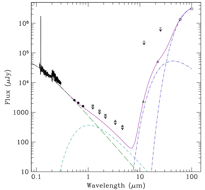
Figure 1. Spectral energy distribution plot for the CS of Abell 65. The IUE spectra, V , R , and I magnitudes (solid circles) at minimum light, 2MASS J , H , and K magnitudes (open squares), WISE fluxes (open triangles), and IRAS fluxes (open circles). All fluxes have been de-reddened assuming E(B - V) = 0.20 . Also shown are model blackbody curves for our resulting CS, companion, and dust component, as well as the combined curve. These are shown without any irradiation contribution, thus should approximately represent the system at minimum light.
