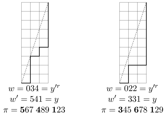
Figure 5: Two lattice paths and the permutations corresponding to the 132-avoiding binary shrubs
